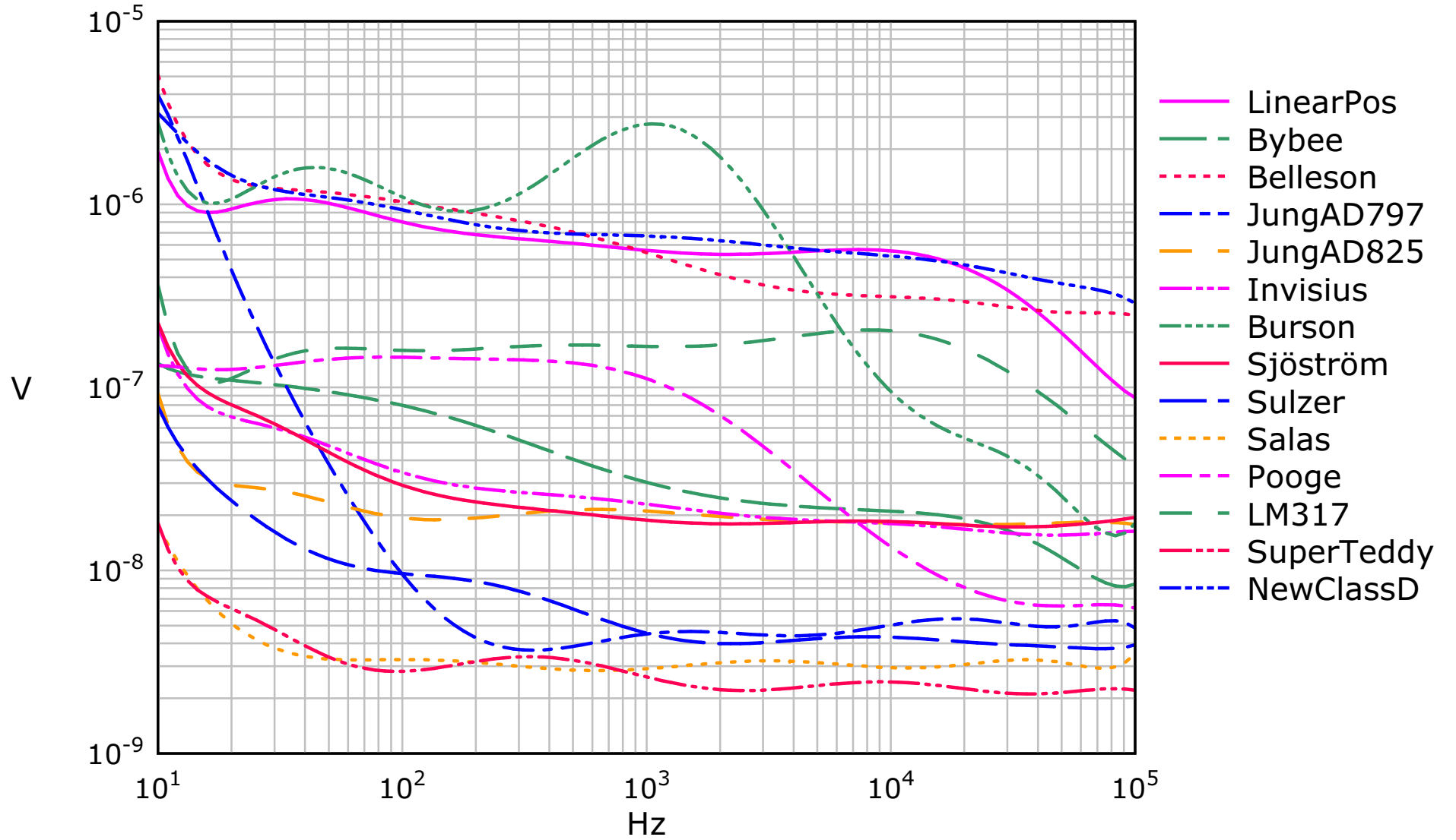
Positive regulator Output Noise (c) Linear Audio / Jack Walton
