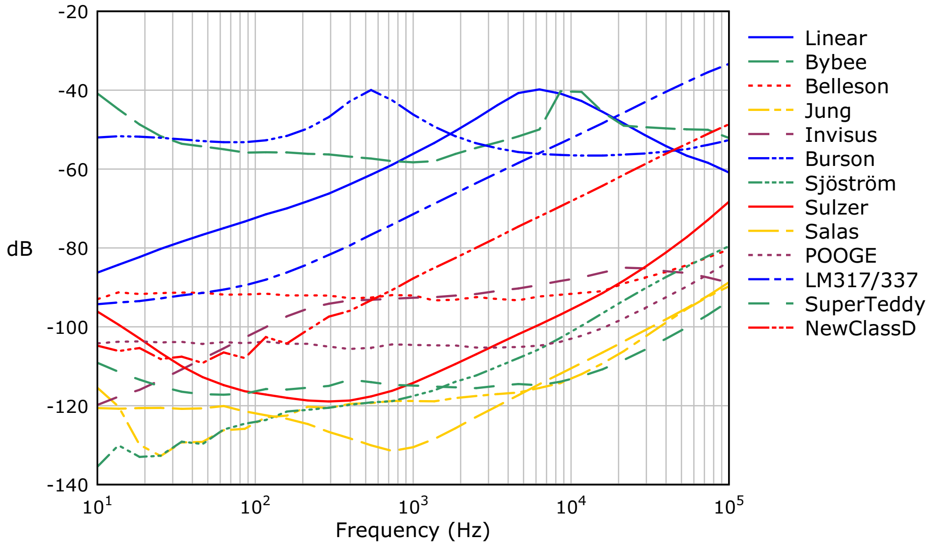
PSRR negative regulators (c) Linear Audio / Jack Walton
