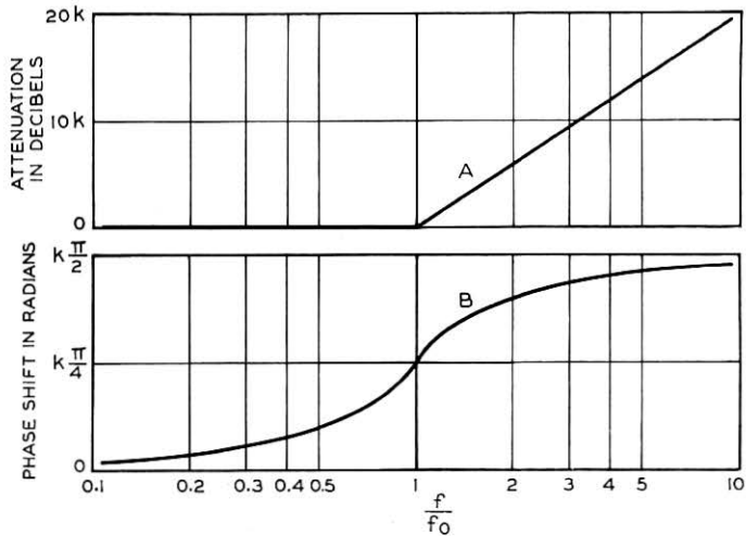
Fig. 5—Phase characteristic corresponding to an attenuation which is constant below a prescribed frequency and has a constant slope above it.
